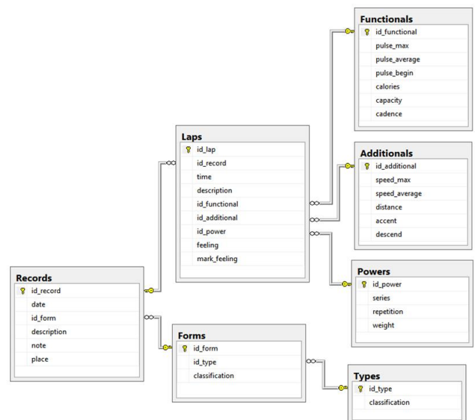
Fig. 1. The database scheme for "Cyclist Diary"
